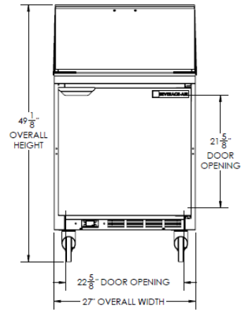
Elevation View
