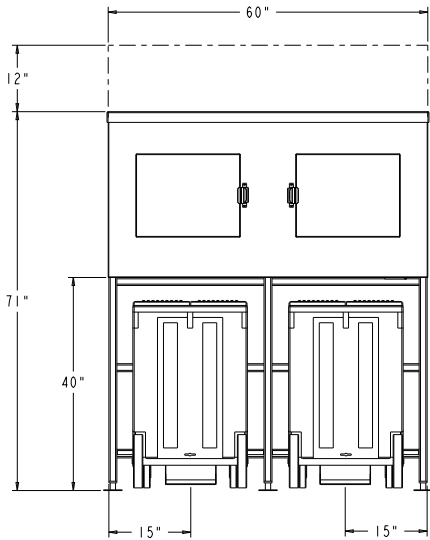
LBCS1360, top, front, side views
