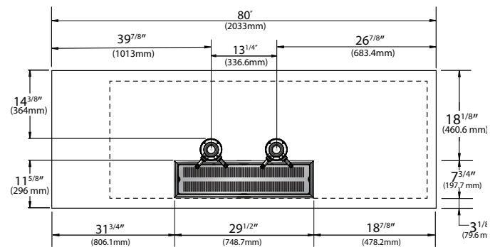
HDD-3-80(-S) Plan View
