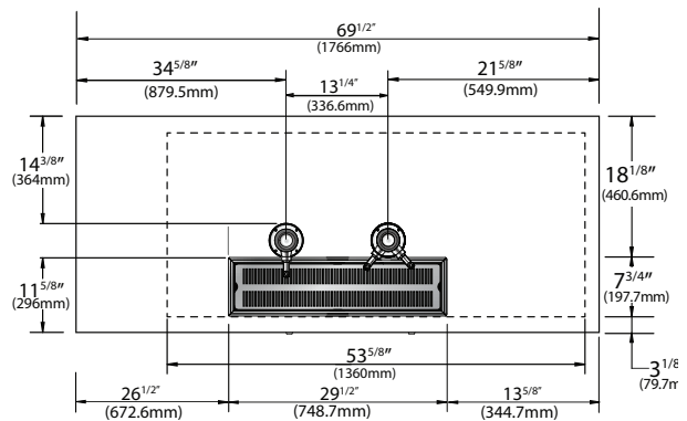
HDD-3-69(-S) Plan View
