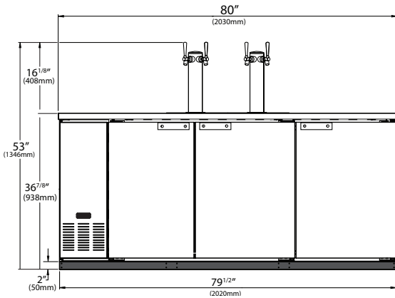
HDD-3-80(-S) Front View
