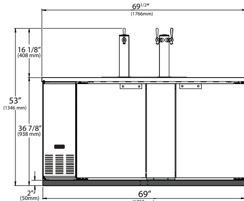
HDD-3-69(-S) Front View
