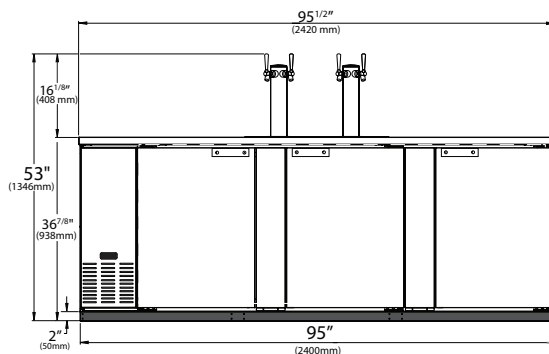
HDD-4-95(-S) Front View
