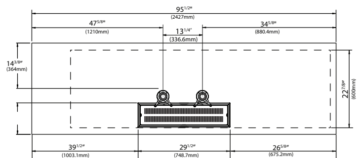
HDD-3-80(-S) Plan View
