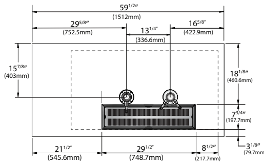
HDD-2-59(-S) Plan View
