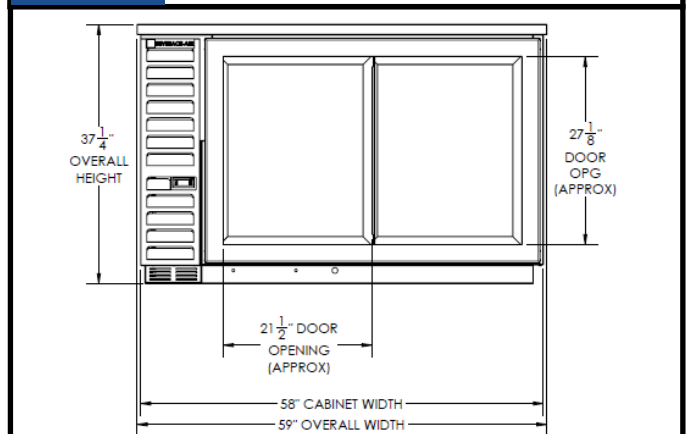
Elevation View
